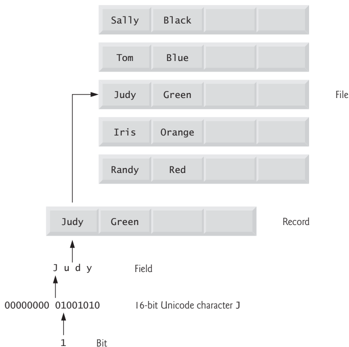
Fig. 1.3 | Data hierarchy.
