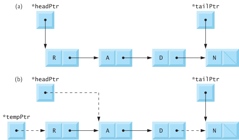
Fig. 12.16 | dequeue operation.
